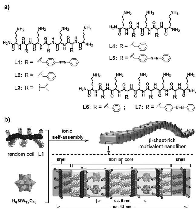
Figure 1. a) Structure of cationic peptides L1–L7. b) Ionic self-assembly of peptide L1 and polyanionic \text{H}_4\text{SiW}_{12}\text{O}_{40} (HSiW).
